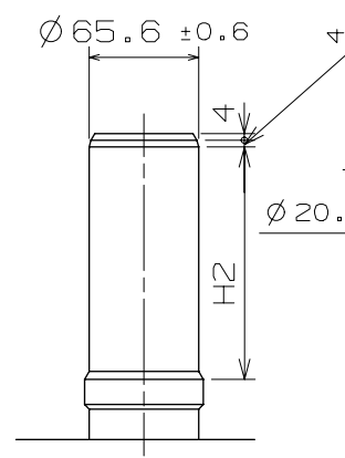
Center wheel
